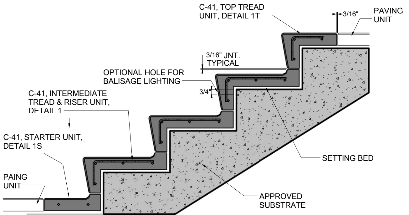
② PARTIAL STAIR CROSS SECTION
