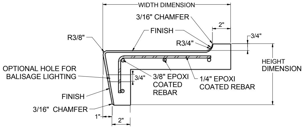
① CROSS SECTION OF INTERMEDIATE TREAD & RISER
