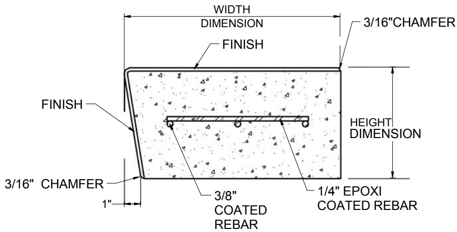
1 TREAD RISER CROSS SECTION
